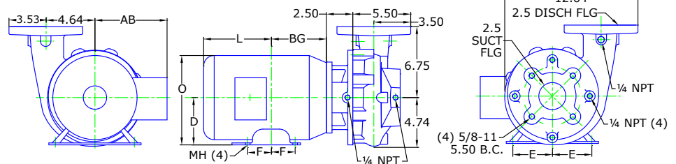
DRAWING DEPICTS JM184 7.5HP ODP MOTOR ALL DIMENSIONS IN INCHES
